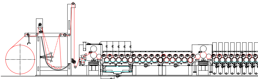
Chain-less mercerizing
